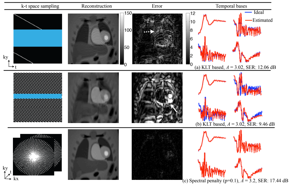
Fig. 5. Comparison of the two-step KLT schemes (two top rows) with the spectrally regularized reconstruction scheme ( p = 0.1 , \lambda_2 = 0 ), shown in the bottom row. The sampling pattern, the peak LV frame of the reconstructed dataset, the corresponding error image (shown at the same scale in all the insets), and the estimated temporal basis functions ( v_i(t) , i = 0 to 3) overlaid on the actual temporal basis functions are shown in each column. Note that the classical KLT based schemes experience a tradeoff between spatial aliasing and accuracy of temporal modeling. The first row correspond to Nt = 41 , where the basis functions are estimated correctly. However, the sparse sampling of outer k-space regions results in spatial aliasing, indicated by the dotted arrow. When the number of phase encodes in training data is reduced to Nt = 5 in the second row, the temporal basis functions fail to capture the dynamics; this often results in inaccurate temporal modeling of the cardiac motion, especially in regions with significant respiratory motion (denoted by the solid arrow). The spectrally regularized reconstruction scheme, along with the radial sampling pattern, is capable of accurately estimating the temporal bases and spatial weights directly from the undersampled data. The significantly decreased errors with the spectral regularization scheme proves the utility in jointly estimating the temporal basis functions and its spatial weights.
