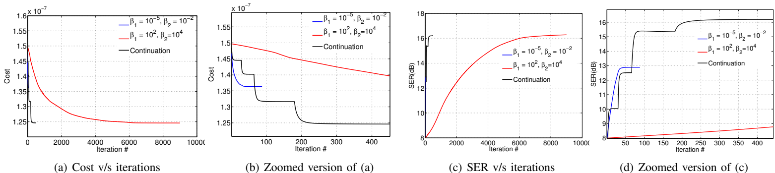
Fig. 3. Convergence of the proposed continuation scheme as a function of \beta_1 and \beta_2 . (a) indicates the evolution of the cost function specified by (10), while (b) is zoomed version of (a). The change in signal to error ratio as a function of the iterations is shown in (c) with its zoomed version in (d). Note that the convergence of the algorithm is very slow if these parameters are chosen as high values, which is needed for the constraints in (12) to be satisfied. In contrast, the algorithm converges very fast, when these parameters are set to low values. However, the solution of \mathcal{D}_{\beta_1, \beta_2} is a poor approximation for the solution of (10). We observe that by properly selecting a continuation scheme, it is possible to significantly improve the convergence rate, while maintaining the accuracy.
