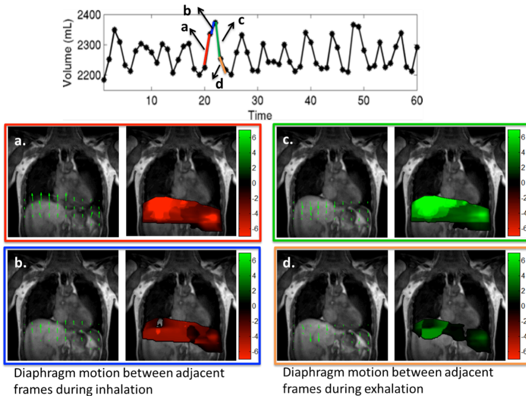
Figure 8: Tracking diaphragm motion using velocity maps: The motion of the diaphragm was tracked at two time points between inspiration shown in (a-b) and two time points between expiration shown in (c-d). The velocity from inspiration to expiration is considered positive (in green) and velocity from expiration to inspiration is considered negative (in red). The velocity field maps and the color-coded velocity maps are shown for all four cases. The change in lung volume shown by blue segment is much lesser than the change in lung volume shown by red segment. This translates to higher diaphragm motion in frames in red segment as compared to the blue segment as seen from the color coded velocity maps in a and b. Similar results were observed during both inspiration and expiration.
