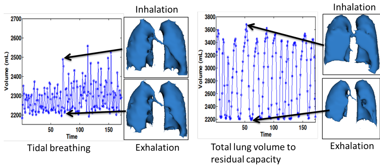
Figure 7: Changes in lung volume as function of time: The figure shows the changes in lung volumes as a function of time in case of tidal breathing maneuver (shown on the left) and deep breathing maneuver from total lung capacity (TLC) to functional residual capacity (FRC) (shown on the right). The segmented lung volumes during peak inhalation and peak exhalation are also shown for both breathing maneuvers. The tidal volume was measured to be approximately 200mL and the normal minute ventilation was around 4L/min. The supine inspiratory capacity was measured to be 1.5L. Note that these numbers are for supine position
