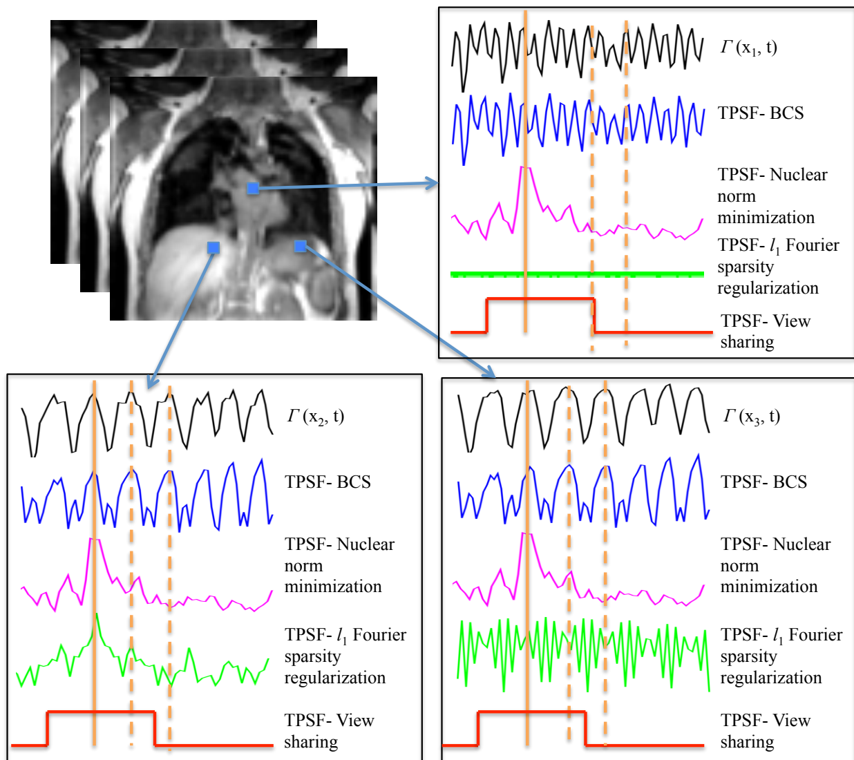
Figure A: Illustrations of different algorithms: The TPSFs at a specific time frame at peak inhalation (shown by solid orange marker) and the underlying signal time profile are shown for three different pixels. The TPSF plots show that all
